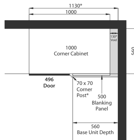
Base Unit: 1000mm (w) Door size: 496mm (w) x 715mm (h) Blanking panel: 500mm (w), can be cut to size
