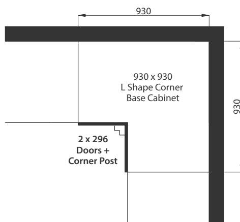
Base Unit: 930 x 930mm L-shape Door size: 2 x 296mm (w) x 715mm (h) Hinges: Unit comes with 170° hinges, each door is hinged independently on the gable.
