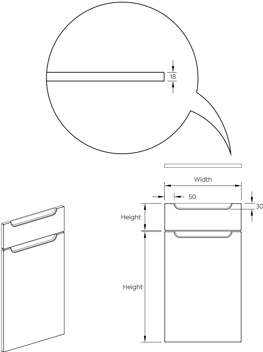
Above example shows: 396w x 140h Drawer 396w x 570h Door
