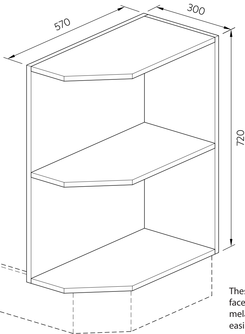
Base Unit
