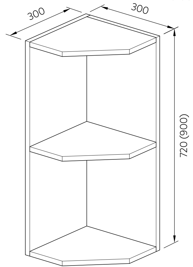
Wall Unit
