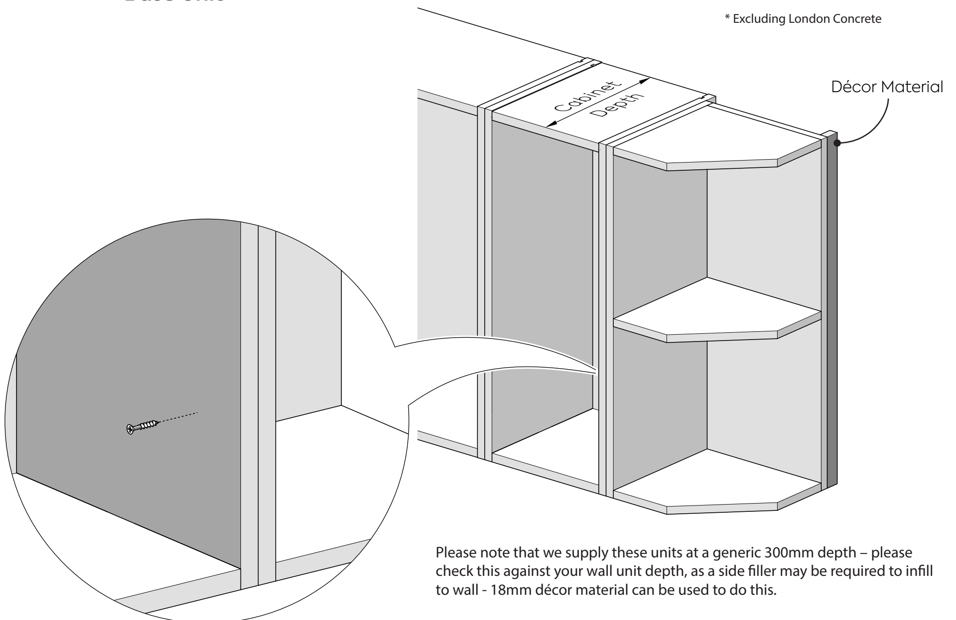
Base Unit
